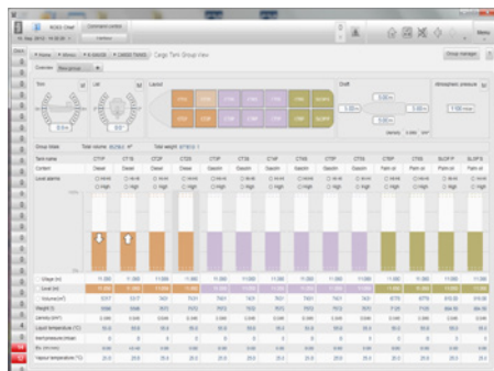
Figure 10: Tank monitoring system mimic (example)
