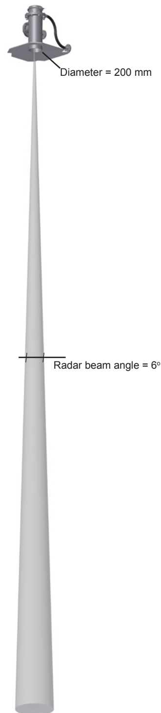
Figure 9: RTG installation on tank socket (example), indicated with free-range radar beam (+/- 3°)
